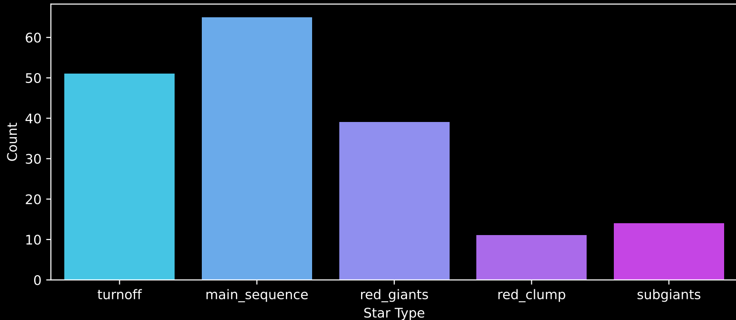
APOGEE DR17 Field: [060+38_MGA] Count plot of Star Type
