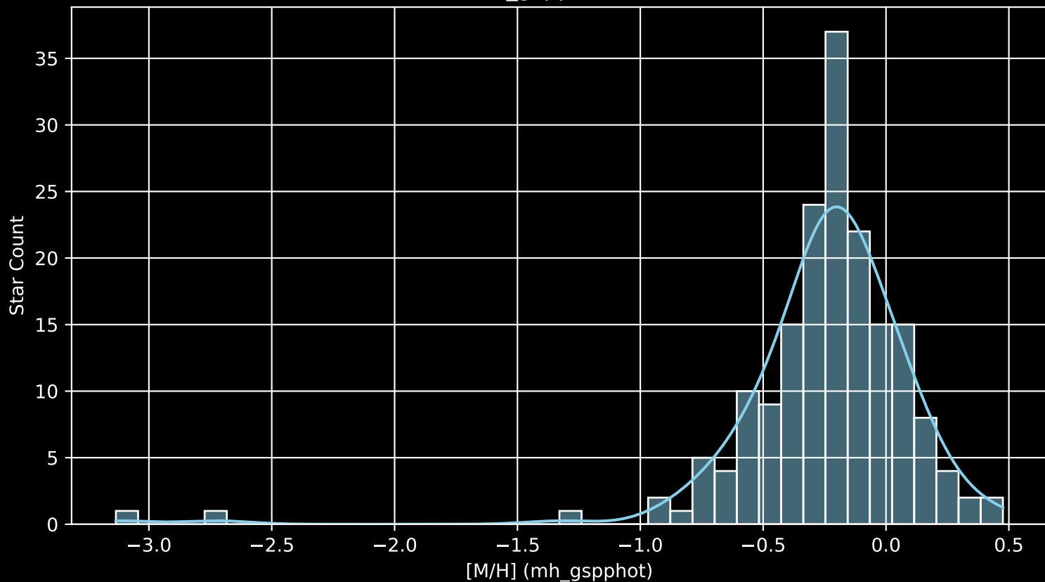
APOGEE DR17 Field: [060+38_MGA [M/H] (mh_gspphot) (n= 178)
