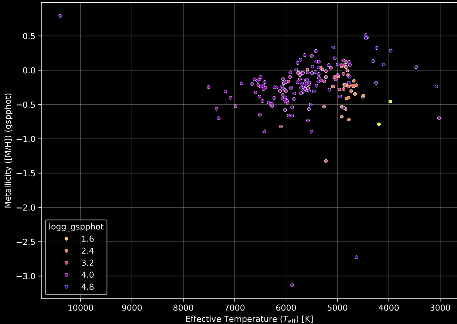
APOGEE DR17 Field: [060+38_MGA] Stellar Population Parameters (n= 180)
