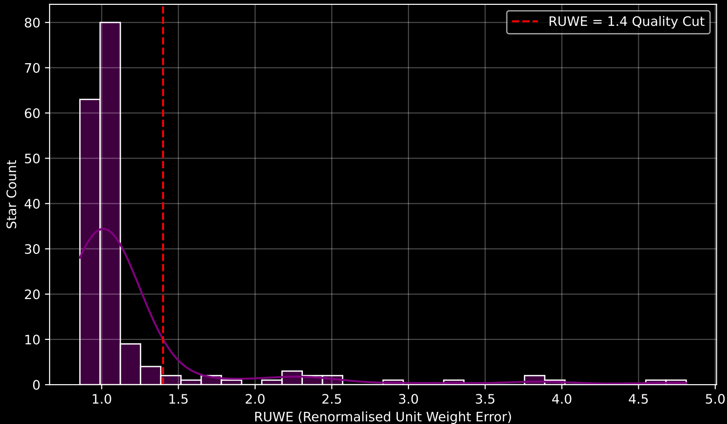
GAPOGEE DR17 Field [060+38_MGA] RUWE Distribution (n= 177)
