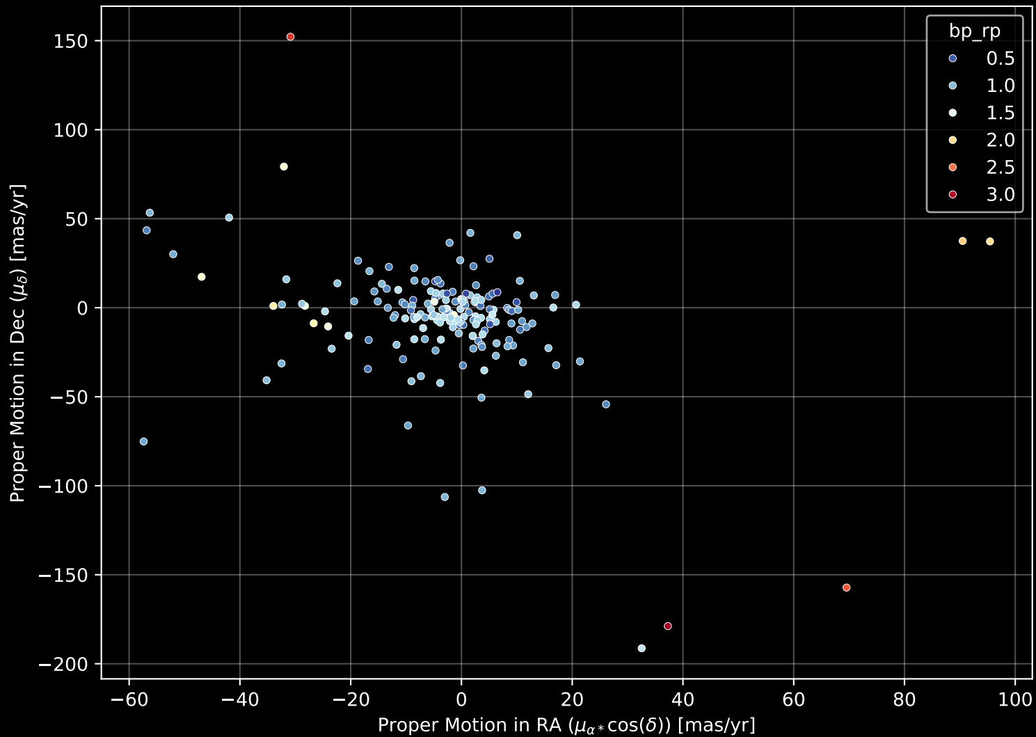
APOGEE DR17 Field: [060+38_MGA] Proper Motion Diagram (n= 180)
