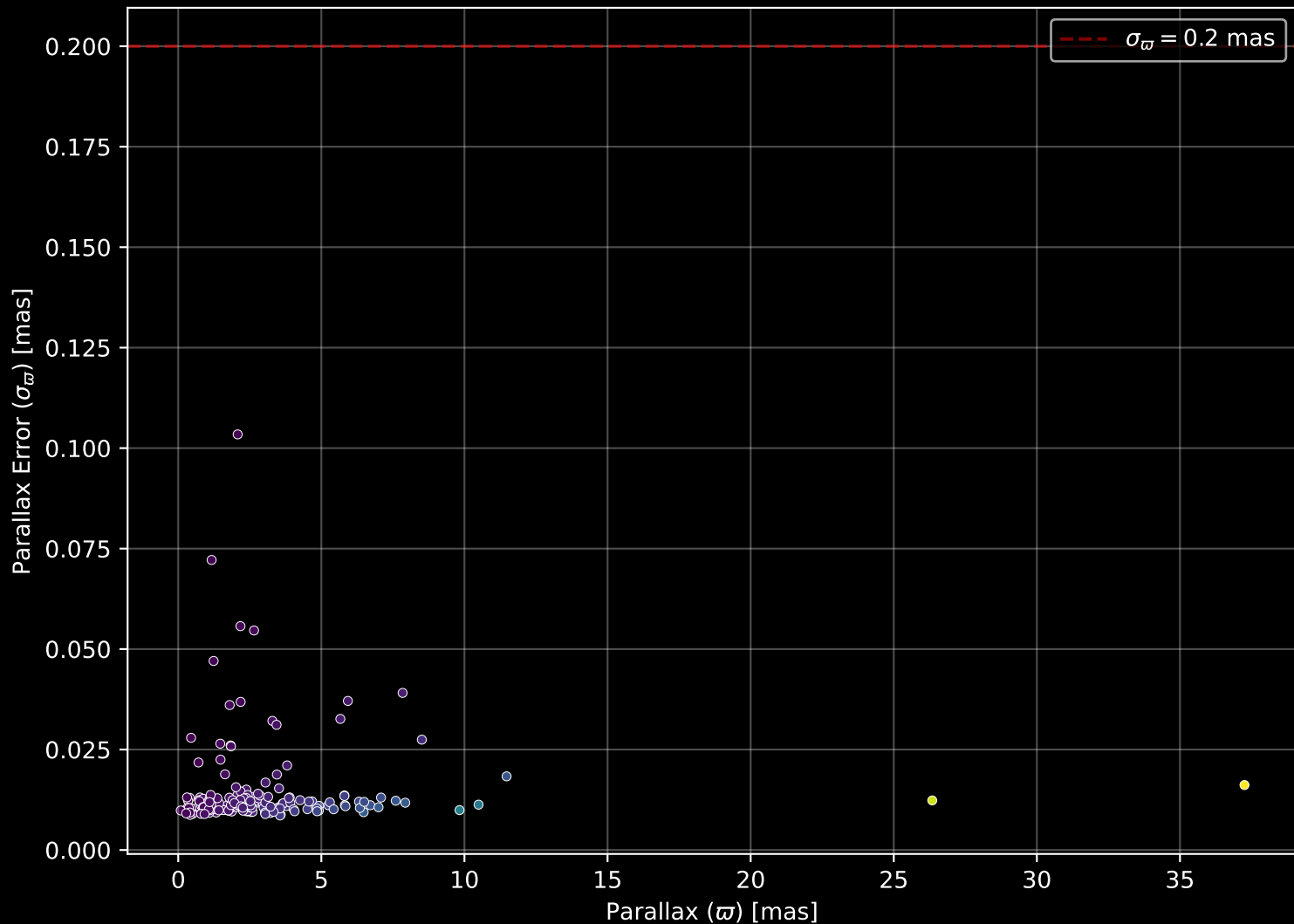
APOGEE DR17 Field: [060+38_MGA] Parallax Quality (n= 180)
